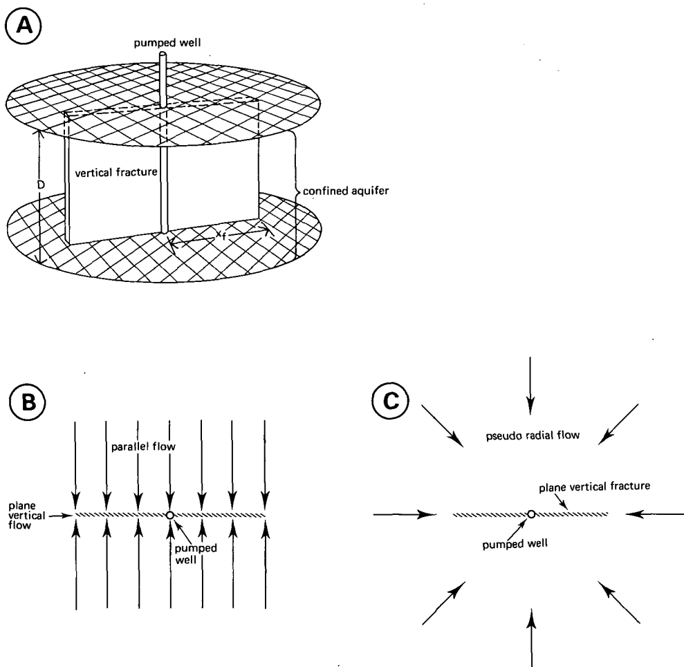
Figure 18.1 A well that intersects a single, vertical, plane fracture of finite length and infinite hydraulic conductivity
