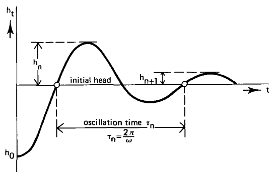
Figure 16.3 Damped harmonic oscillation
