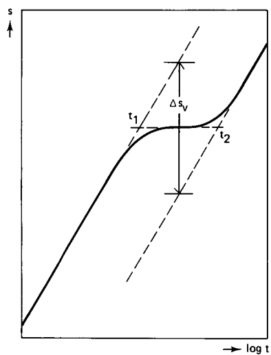
Figure 17.4 Semi-log time-drawdown plot for an observation well in a fractured rock formation of the double-porosity type
