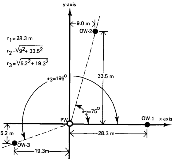
Figure 8.2 Location of the pumped well and observation wells (Papadopolus pumping test, Example 8.1)
