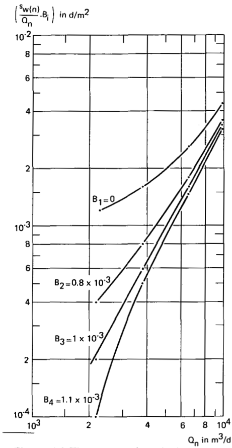
Figure 14.6 The Rorabaugh method
