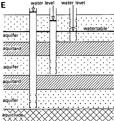
Figure 1.1 Different types of aquifers
