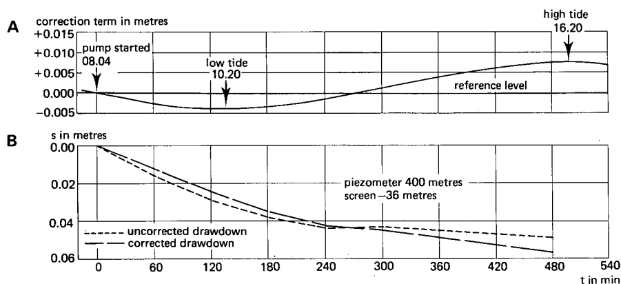
Figure 2.10 Correction of data for tidal influence
