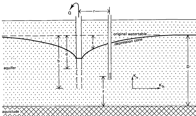
Figure 10.7 The geometric parameters of Neuman's method for a well partially penetrating an unconfined aquifer
