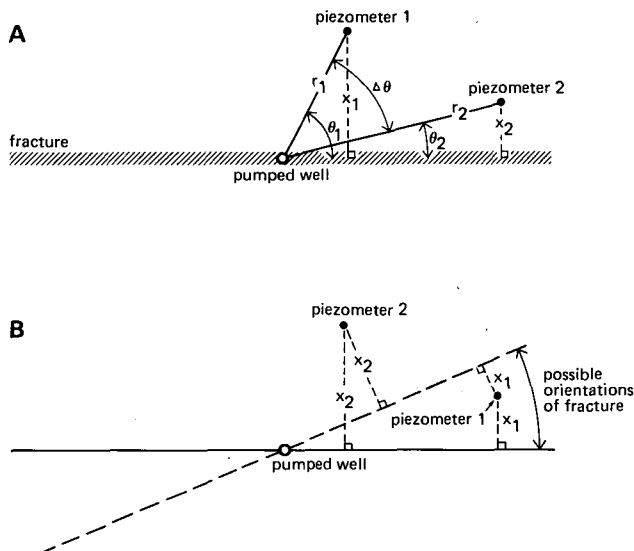
Figure 2.6 Piezometer arrangement near a fracture:
