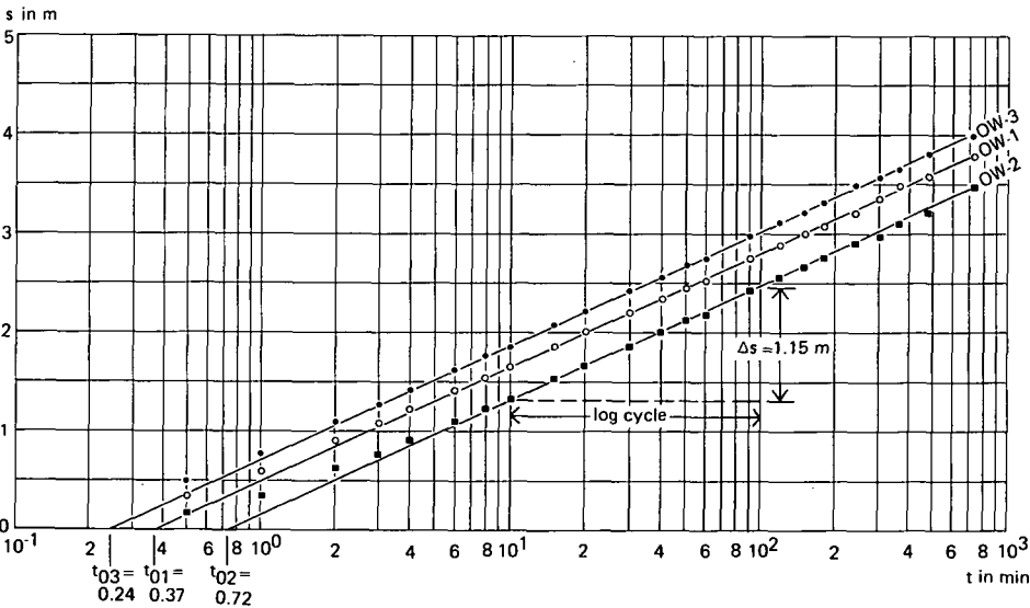
Figure 8.3 Analysis of data from the Papadopolus pumping test with the Jacob method
