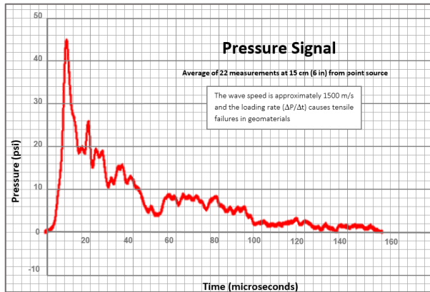
Figure 5. Shock Wave Characteristics of an EHS tool at a distance of 15 cm (6 in) from the point source. A very sharp peak is seen in the 5 – 10 microsecond range.
