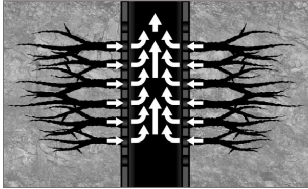
Figure 4. The removal of organics and scales up to 2 m (6.5 ft) from the borehole reduce the skin value and allow for improved fluid flow into the borehole.
